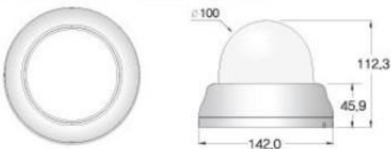
DOME CAMERA DIMENSIONS (mm)
